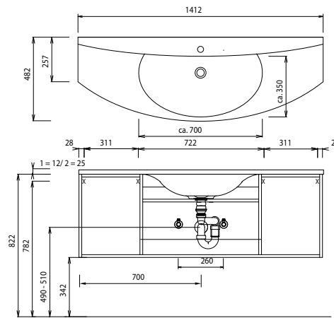
SWM/SWG 8140
