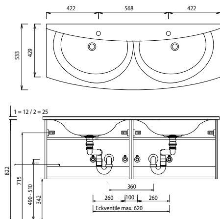
SWM 814D
