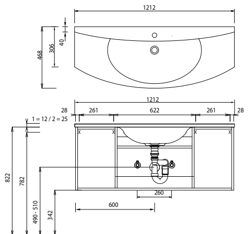
SWM/SWG 8120
