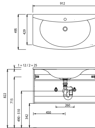
SWM/SWG 8090
