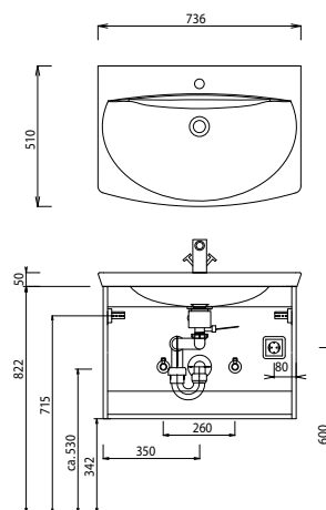
SWM 6270
